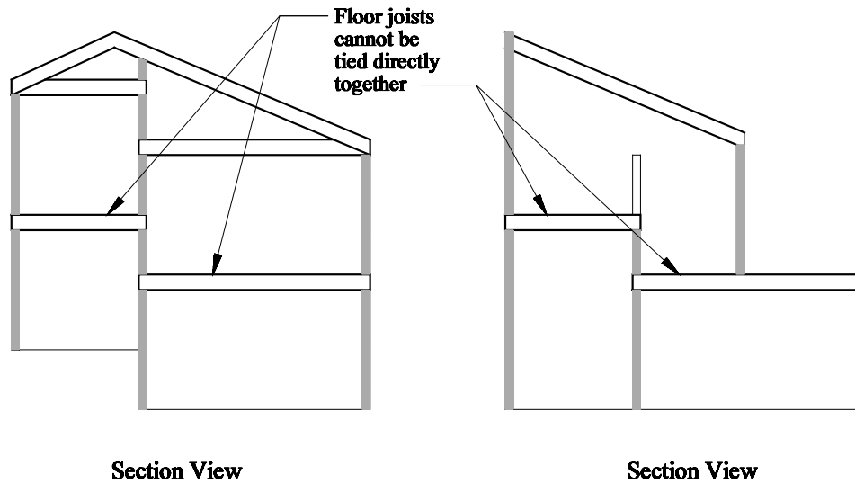
Figure 12.4-7 Vertical Offset Irregularity.
