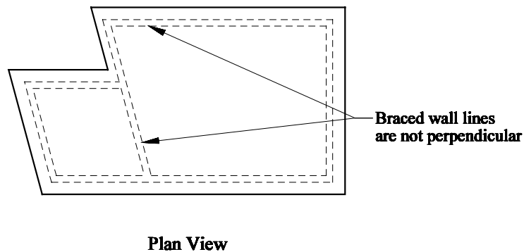
Figure 12.4-8 Non perpendicular Walls Irregularity.
