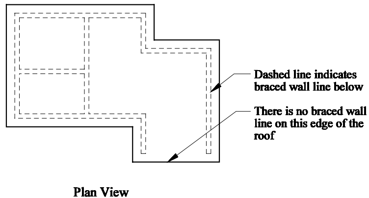
Figure 12.4-4 Unsupported Diaphragm Irregularity.
