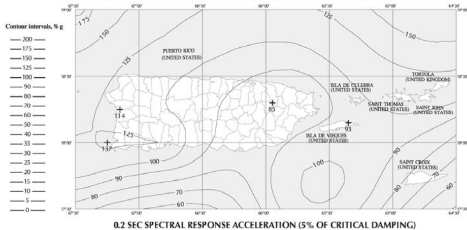
FIGURE 3.3-13 MAXIMUM CONSIDERED EARTHQUAKE GROUND MOTION FOR PUERTO RICO, CULEBRA, VIEQUES, ST. THOMAS, ST. JOHN, AND ST. CROIX OF 0.2 AND 1.0 SEC SPECTRAL RESPONSE ACCELERATION (5% OF CRITICAL DAMPING), SITE CLASS B
