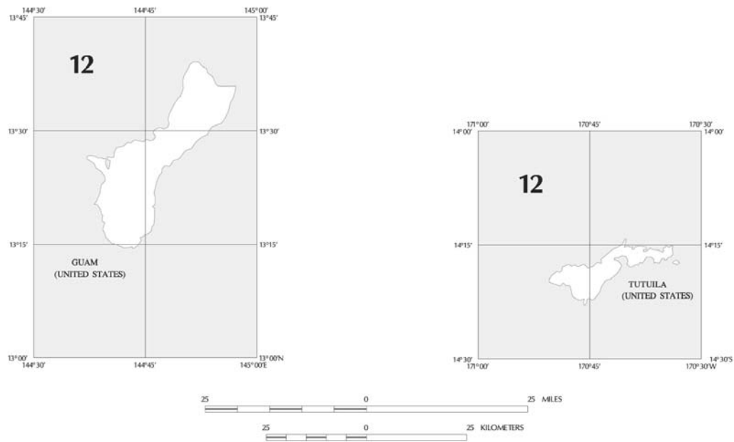
FIGURE 3.3-21 LONG-PERIOD TRANSITION PERIOD, T_1 (sec), FOR GUAM AND TUTUILA
