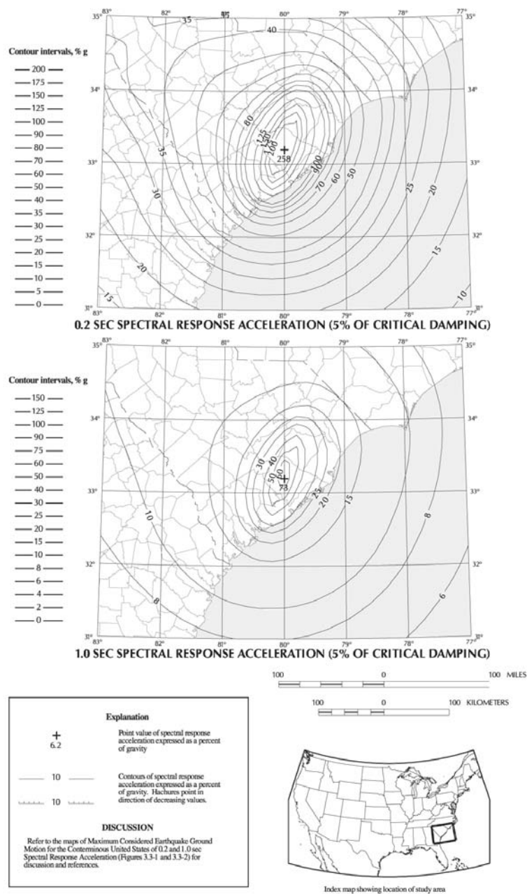
FIGURE 3.3-9 MAXIMUM CONSIDERED EARTHQUAKE GROUND MOTION FOR REGION 4 OF 0.2 AND 1.0 SEC SPECTRAL RESPONSE ACCELERATION (5% OF CRITICAL DAMPING), SITE CLASS B
