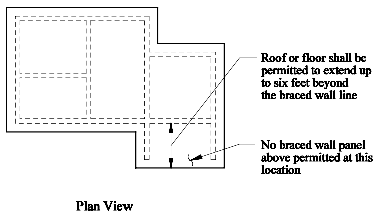
Figure 12.4-5 Permitted Diaphragm Extension.
