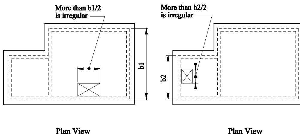
Figure 12.4-9 Diaphragm Opening Irregularity.
