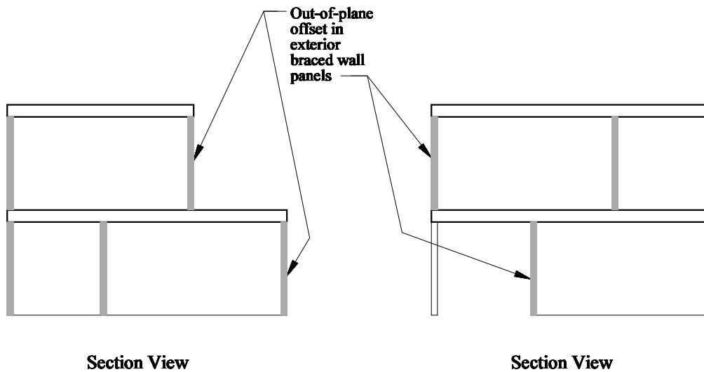
Figure 12.4-2 Out-of-Plane Offset Irregularity.
