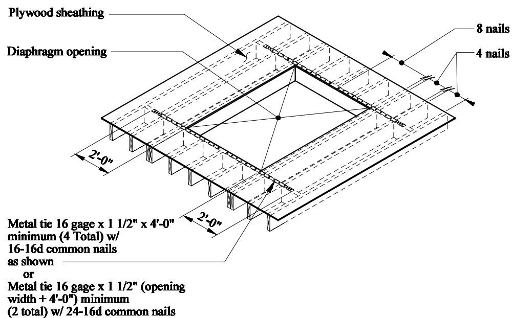
Figure 12.4 -11 Detail for Diaphragm Opening.
