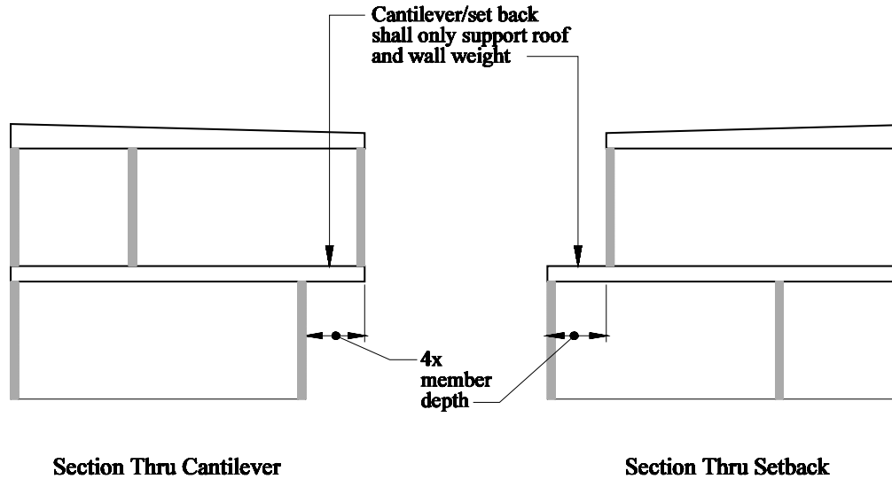
Figure 12.4-3 Permitted Cantilevers and Setbacks.
