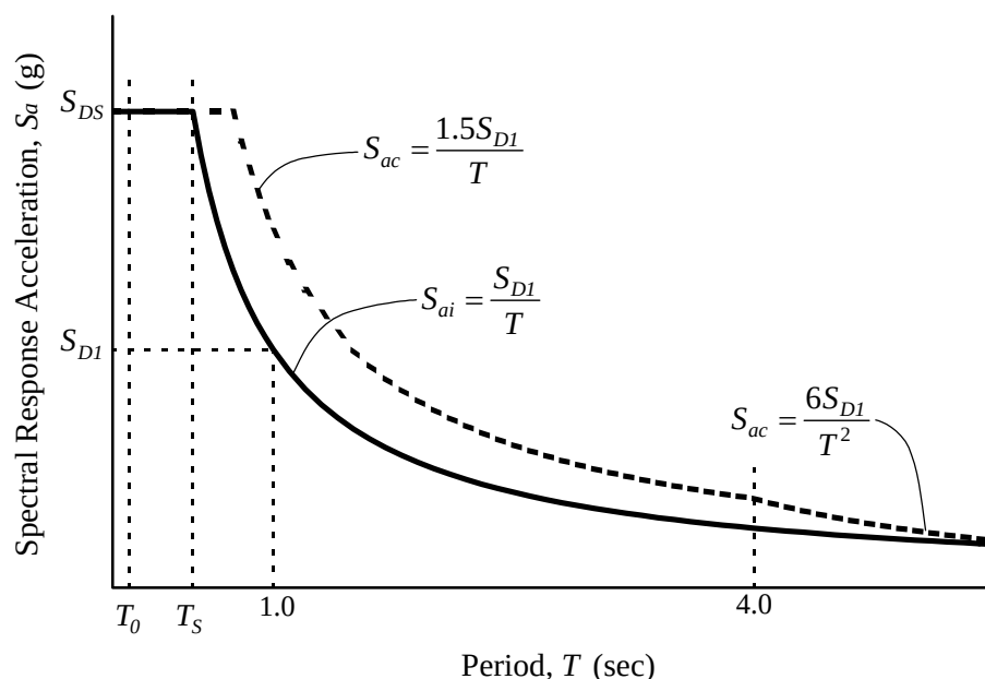
Figure 14.4-1 Design Response Spectra for Ground-supported Liquid Storage Tanks
