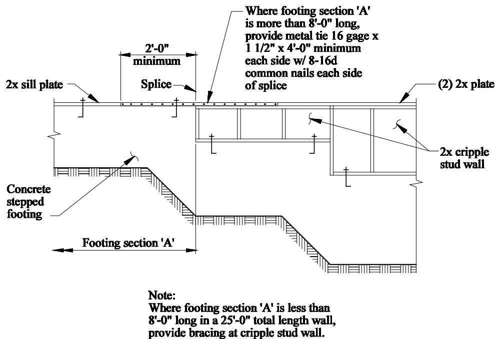
Figure 12.4-10 Detail for Stepped Foundation.
