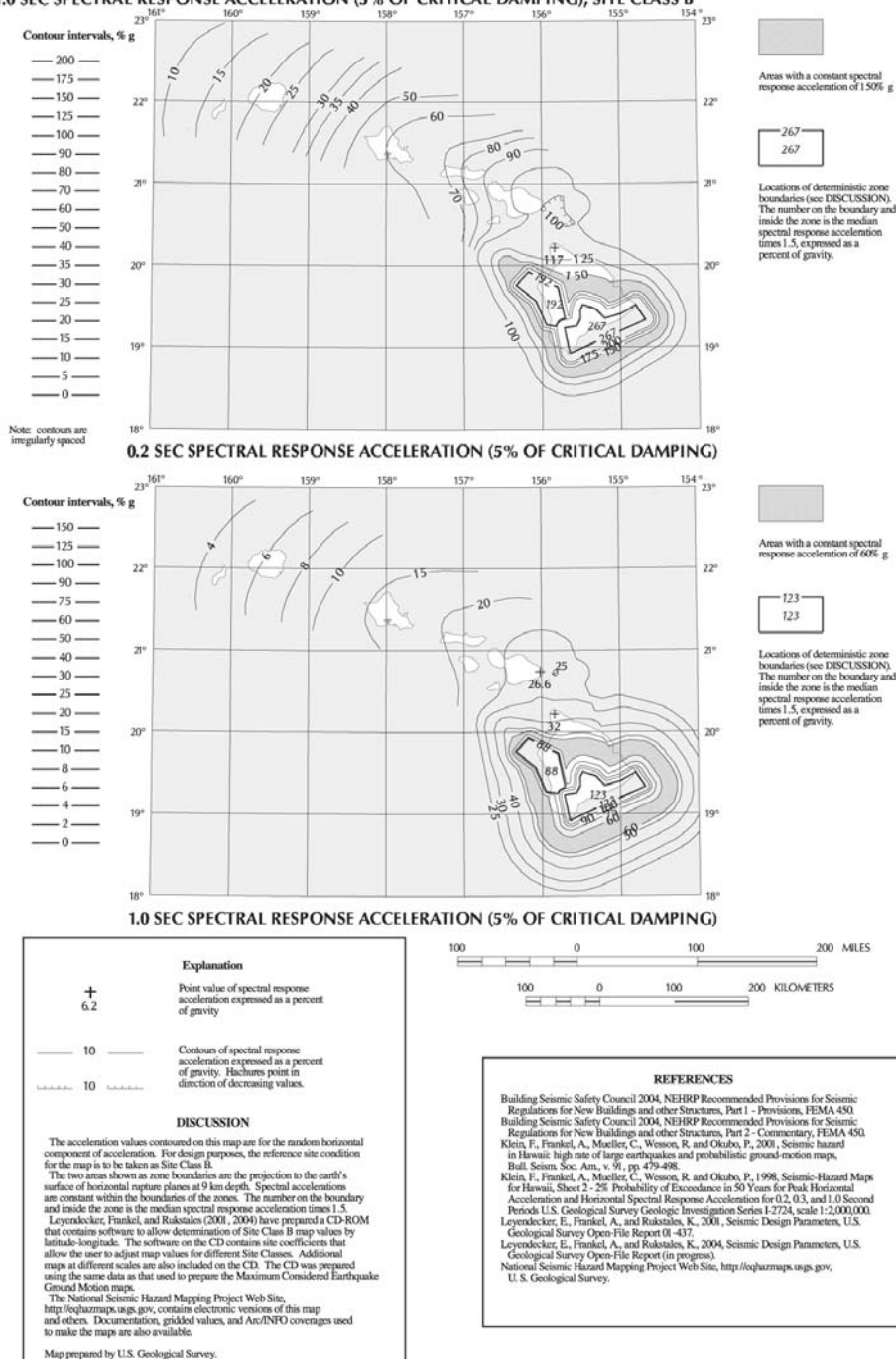
FIGURE 3.3-10 MAXIMUM CONSIDERED EARTHQUAKE GROUND MOTION FOR HAWAII OF 0.2 AND 1.0 SEC SPECTRAL RESPONSE ACCELERATION (5% OF CRITICAL DAMPING), SITE CLASS B
