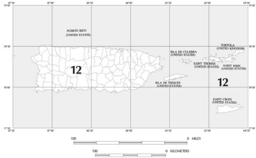
FIGURE 3.3-20 LONG-PERIOD TRANSITION PERIOD, T_1 (sec), FOR PUERTO RICO, CULEBRA, VIEQUES, ST. THOMAS, ST. JOHN, AND ST. CROIX
