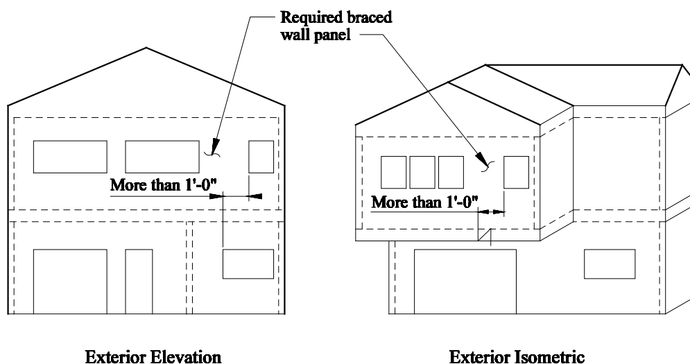
Figure 12.4-6 Opening in Wall Below Irregularity.
