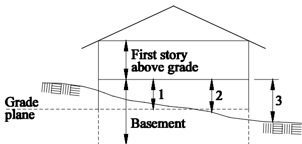
Figure 12.4-1 Definition of Story Above Grade.
